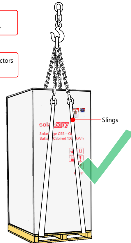
Packaged Battery Cabinet Crane Transportation
