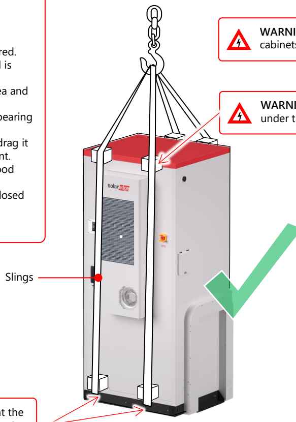
Standalone Battery Cabinet Crane Transportation
